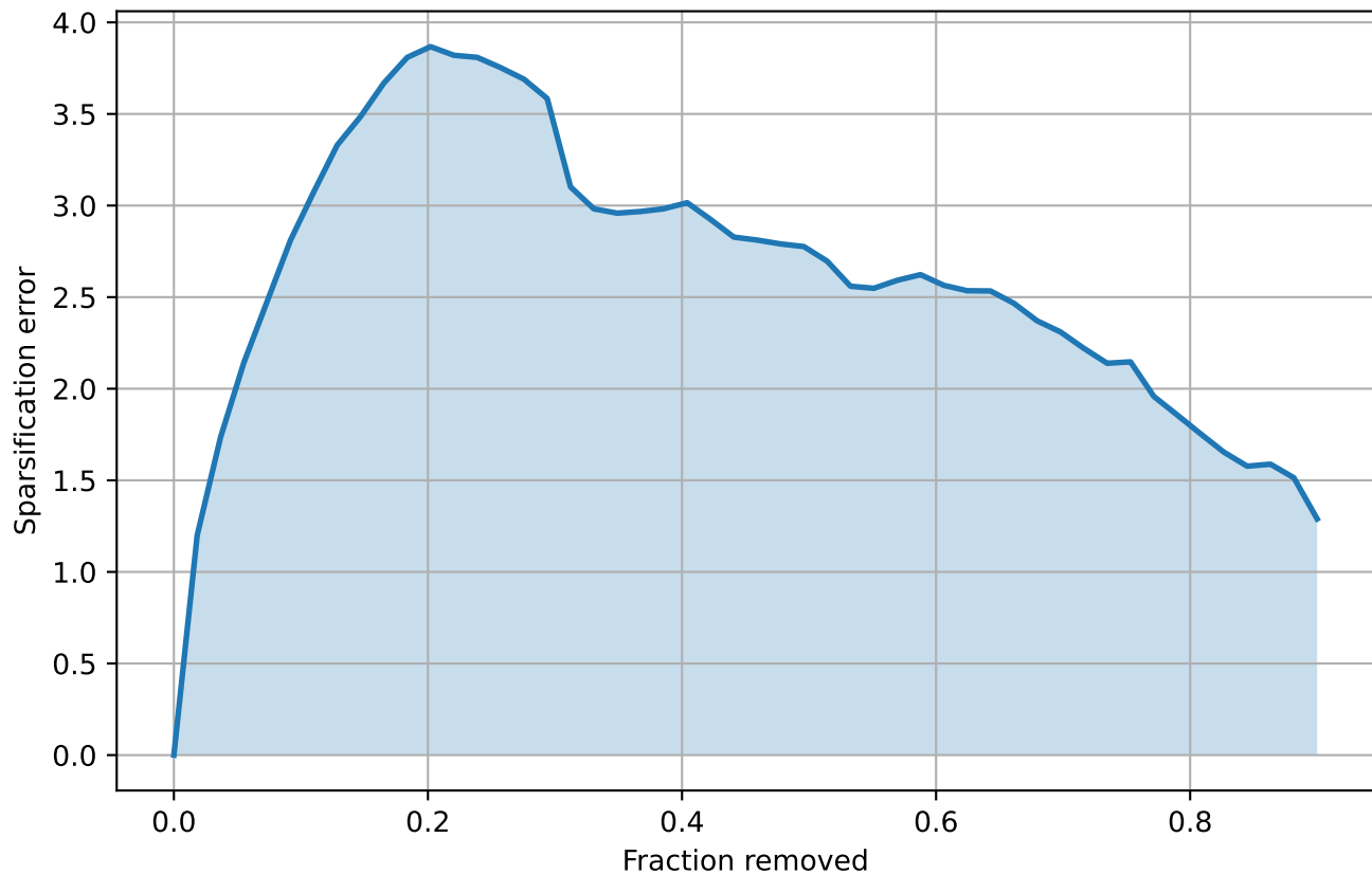
BPIC20ID: Sparsification Error Curve AUSE=2.3740 AURG=6.2153
